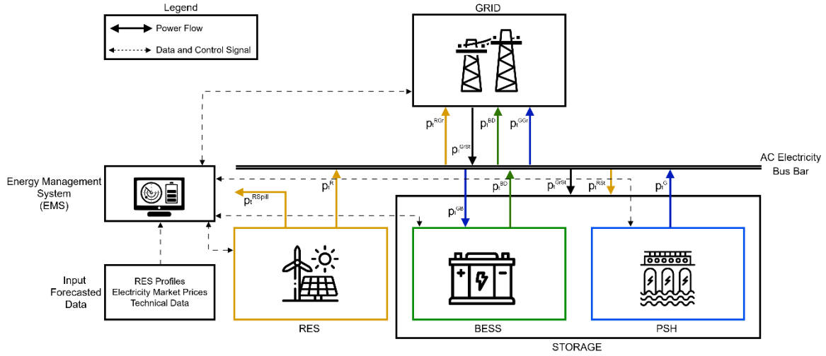
Fig. 2. Schematic representation of the grid-connected co-located hybrid asset under investigation in Model C, consisting of a pumped storage hydro (PSH) system, a battery energy storage system (BESS), and non-dispatchable renewable energy sources (RES).
